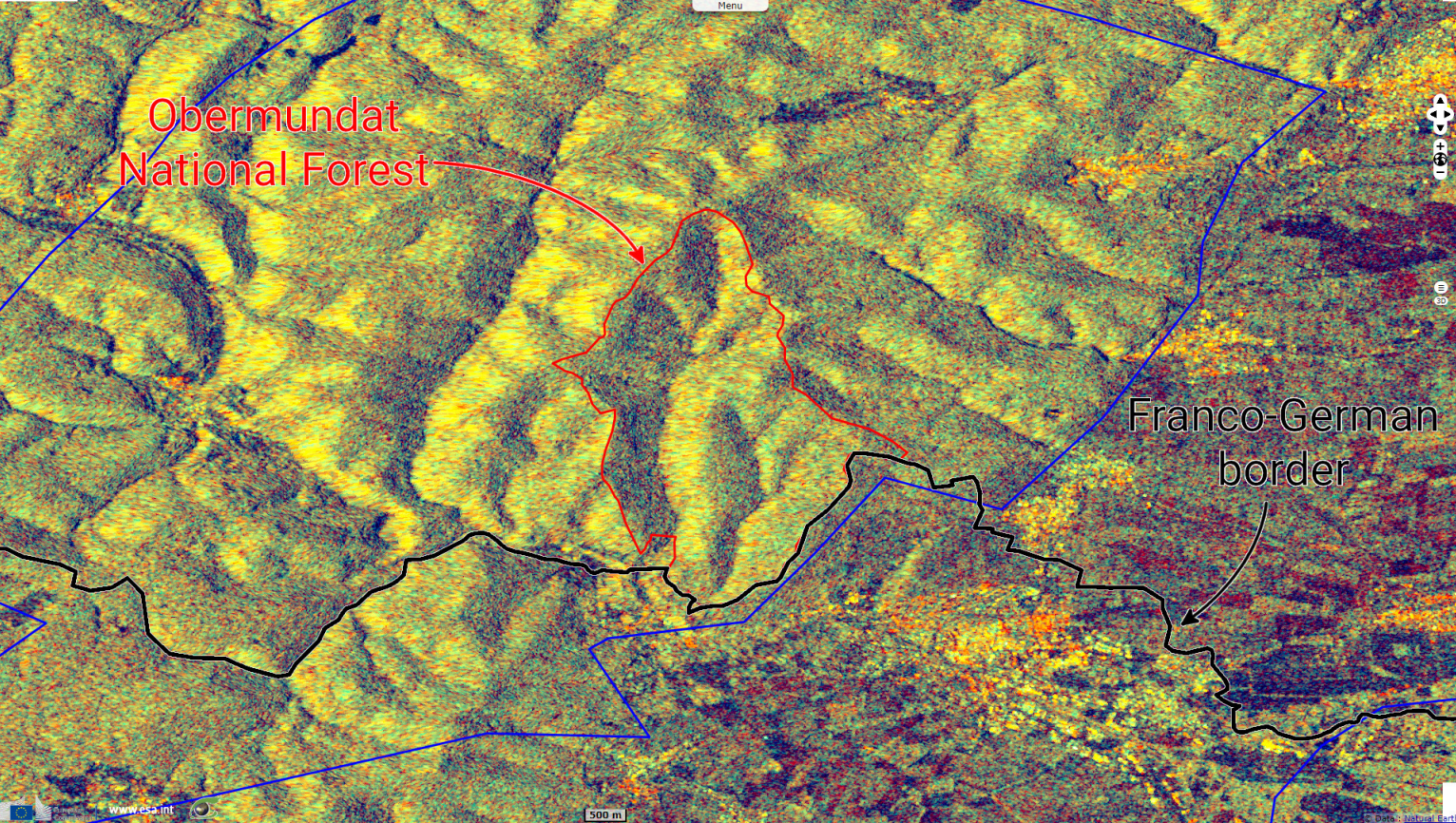
Fig. 3 - S1 (07.10.2023) - The Obermundat forest is a France-owned land in Germany managed by the "Office National des Forêts". 2D view
