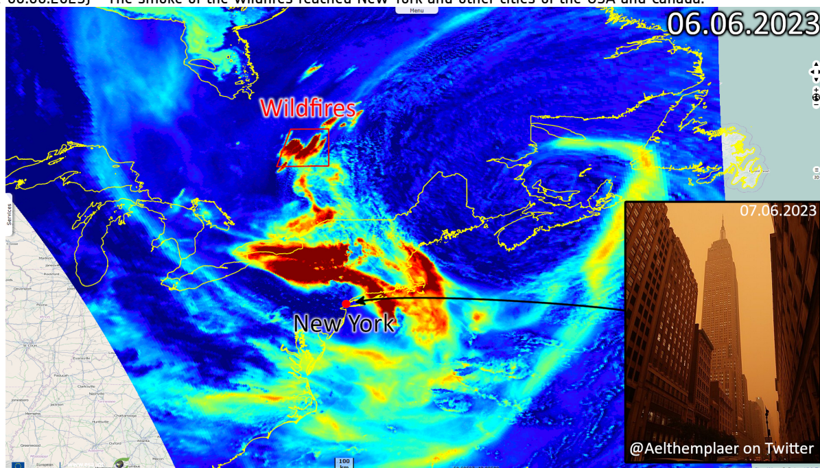
Fig. 2 - S5P (02-06.06.2023) - The smoke of the wildfires reached New York and other cities of the USA and Canada.
