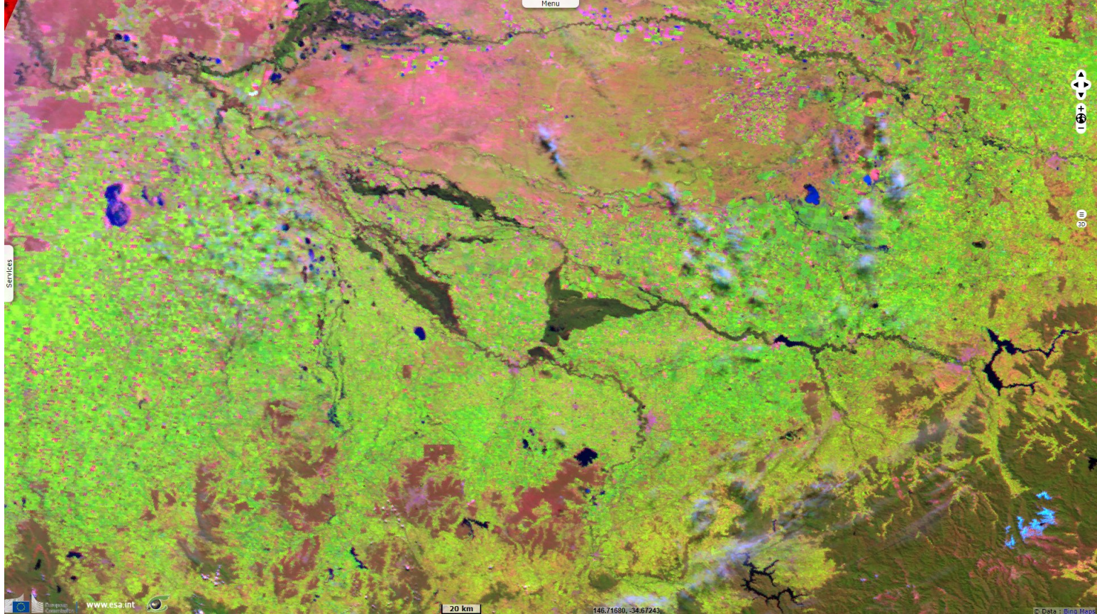
Fig. 2 - S3 OLCI + SLSTR (16-18.10.2022) - There were more than 90 flood warnings active across Victoria state, south-eastern Australia.
