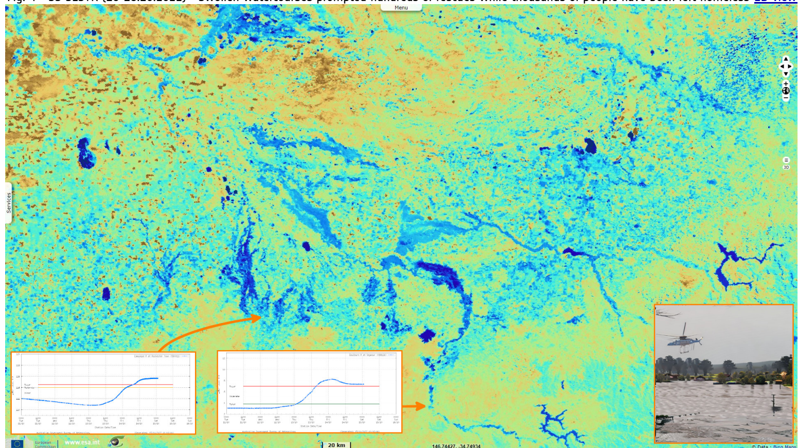
Fig. 4 - S3 SLSTR (16-18.10.2022) - Swollen watercourses prompted hundreds of rescues while thousands of people have been left homeless 2D view
