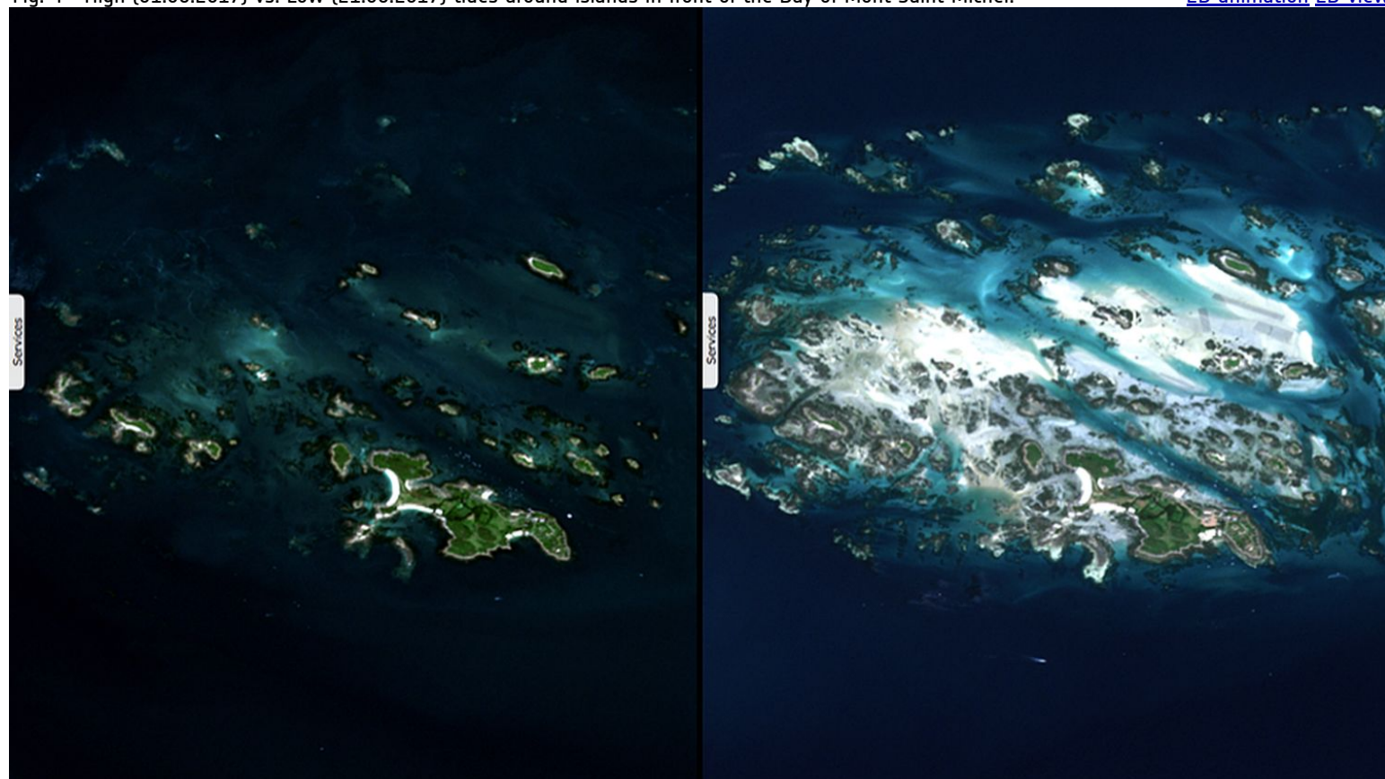
Fig. 4 - High (01.06.2017) vs. Low (21.06.2017) tides around islands in front of the Bay of Mont Saint Michel.
