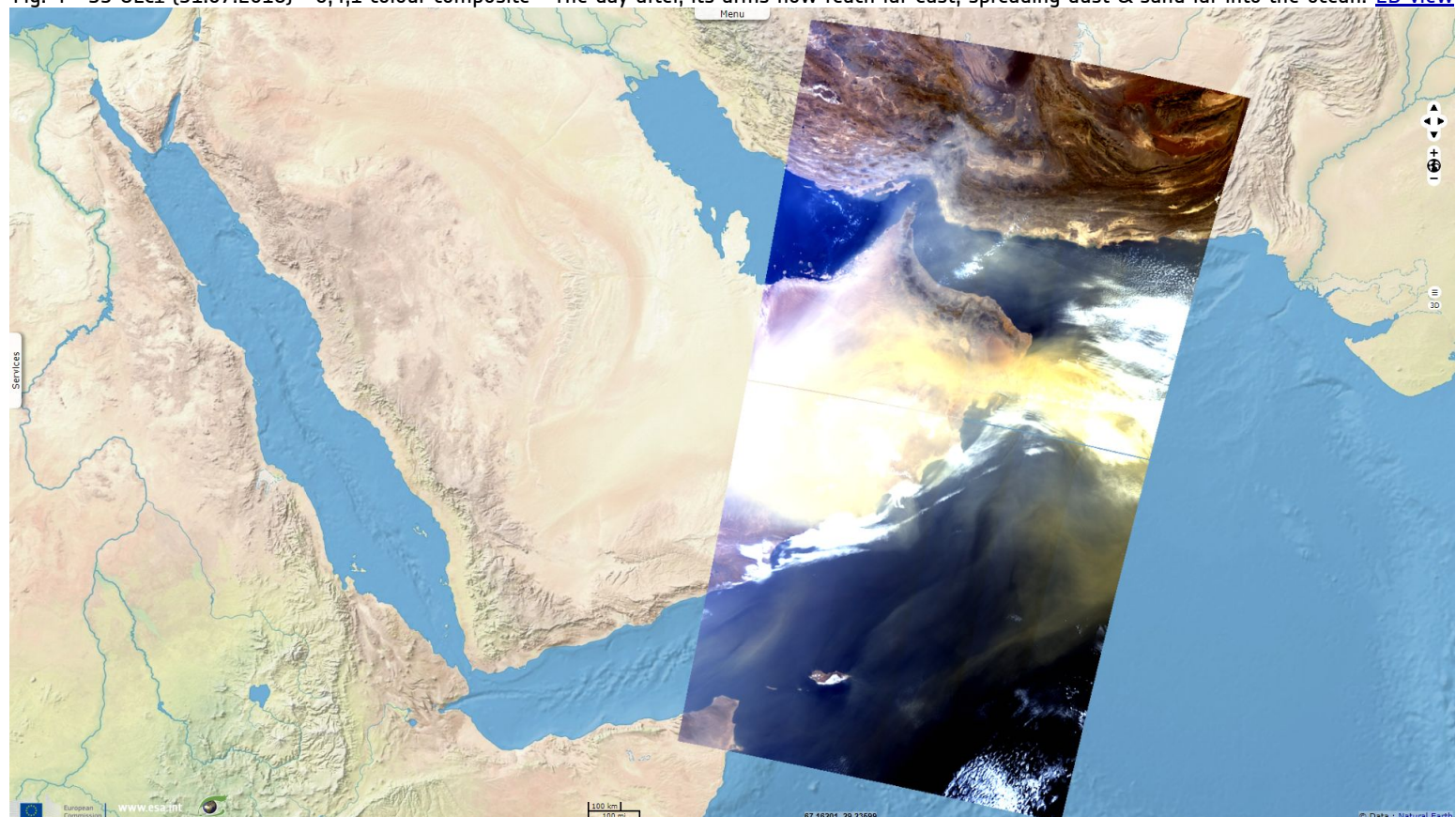
Fig. 4 - S3 OLCI (31.07.2018) - 6,4,1 colour composite - The day after, its arms now reach far east, spreading dust & sand far into the ocean.
