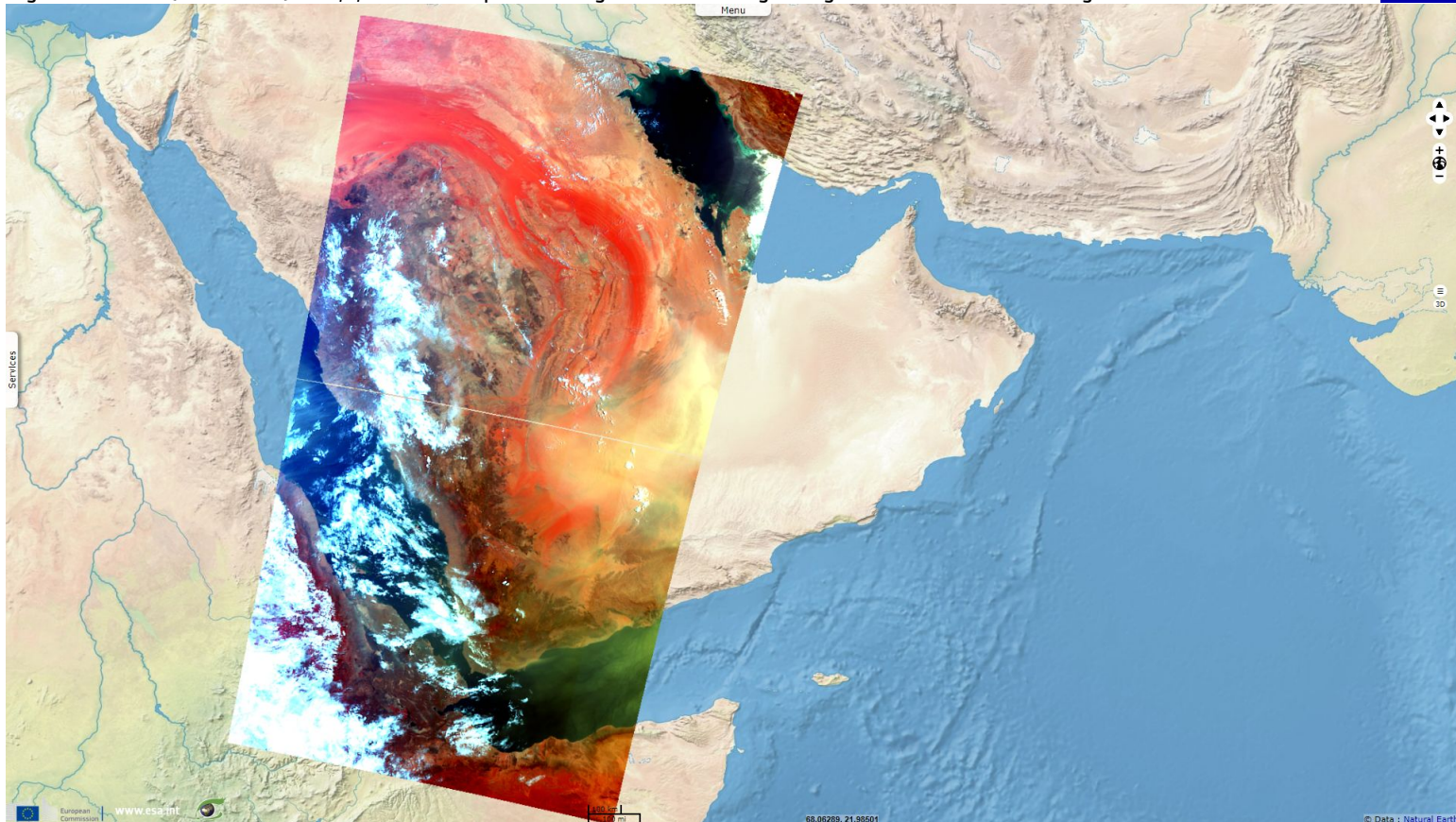
Fig. 2 - S3 OLCI (30.07.2018) - 6,4,1 colour composite - Larger view of the storm spiral acquired the following day.
