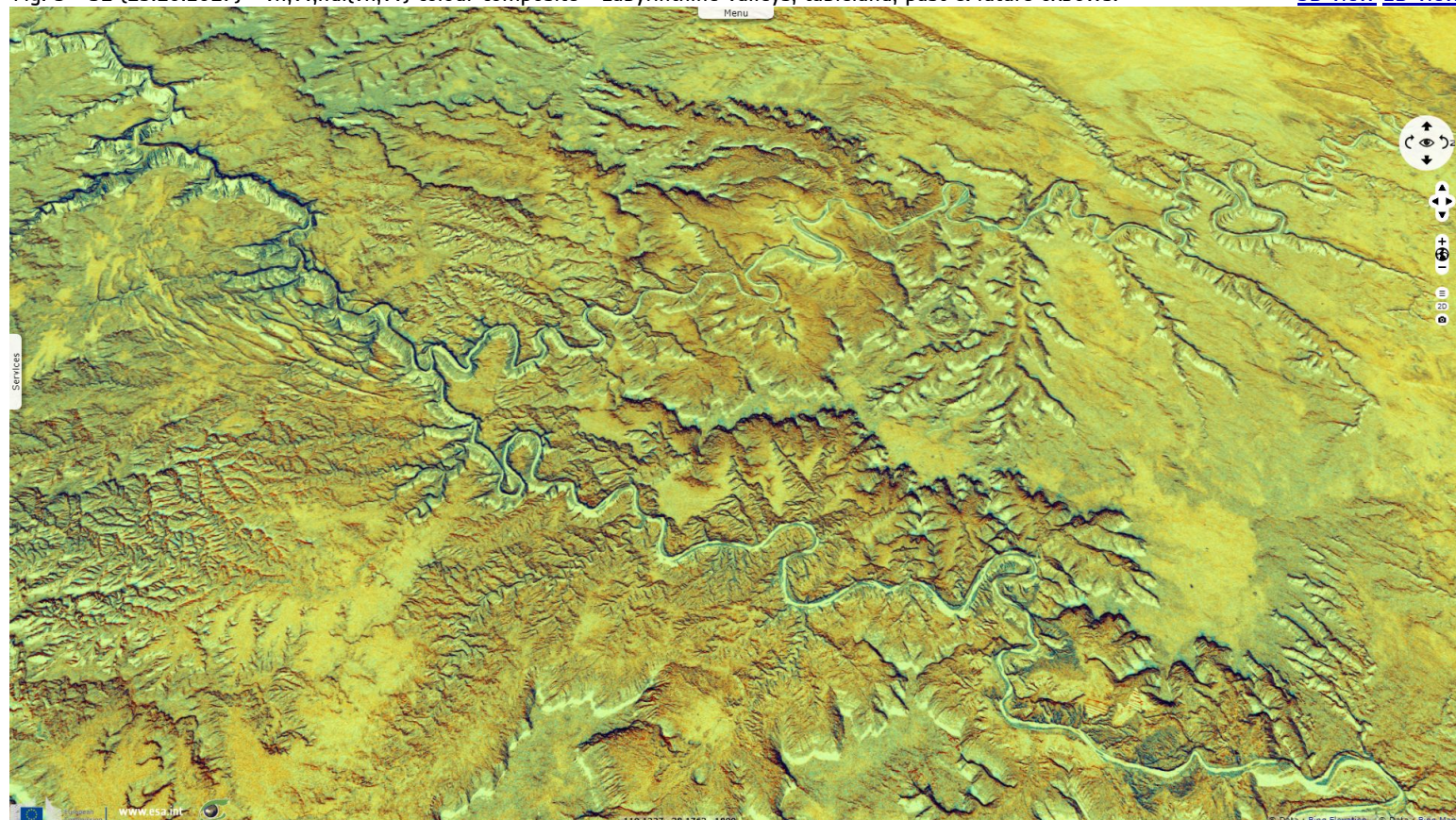
Fig. 4 - S2 (12.10.2017) - 11,8,2 colour composite - The eye of Upheaval Dome shows in Canyonlands National Park.
