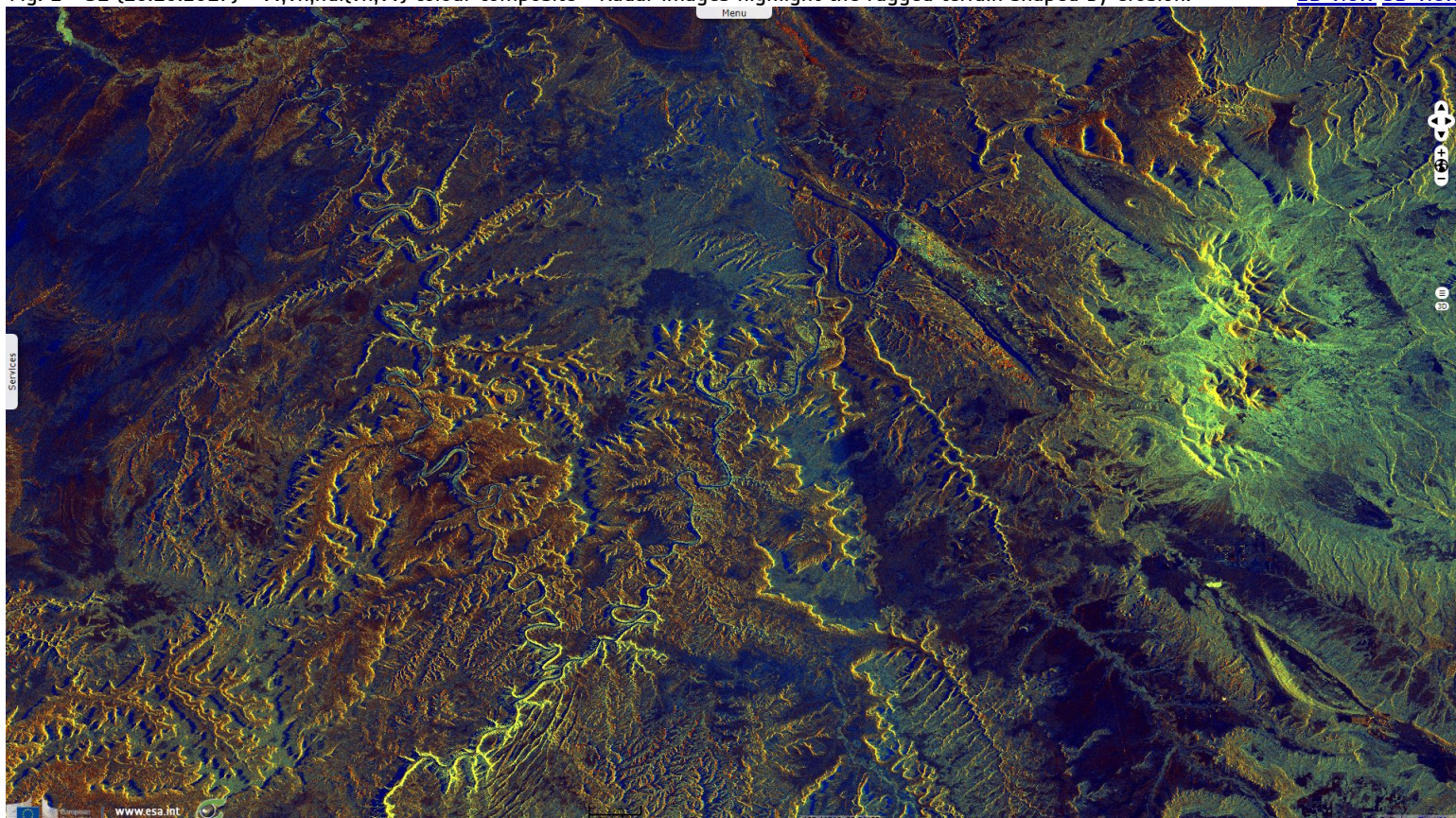
Fig. 2 - S1 (16.10.2017) - vv,vh,ndi(vh,vv) colour composite - Radar images highlight the rugged terrain shaped by erosion.
